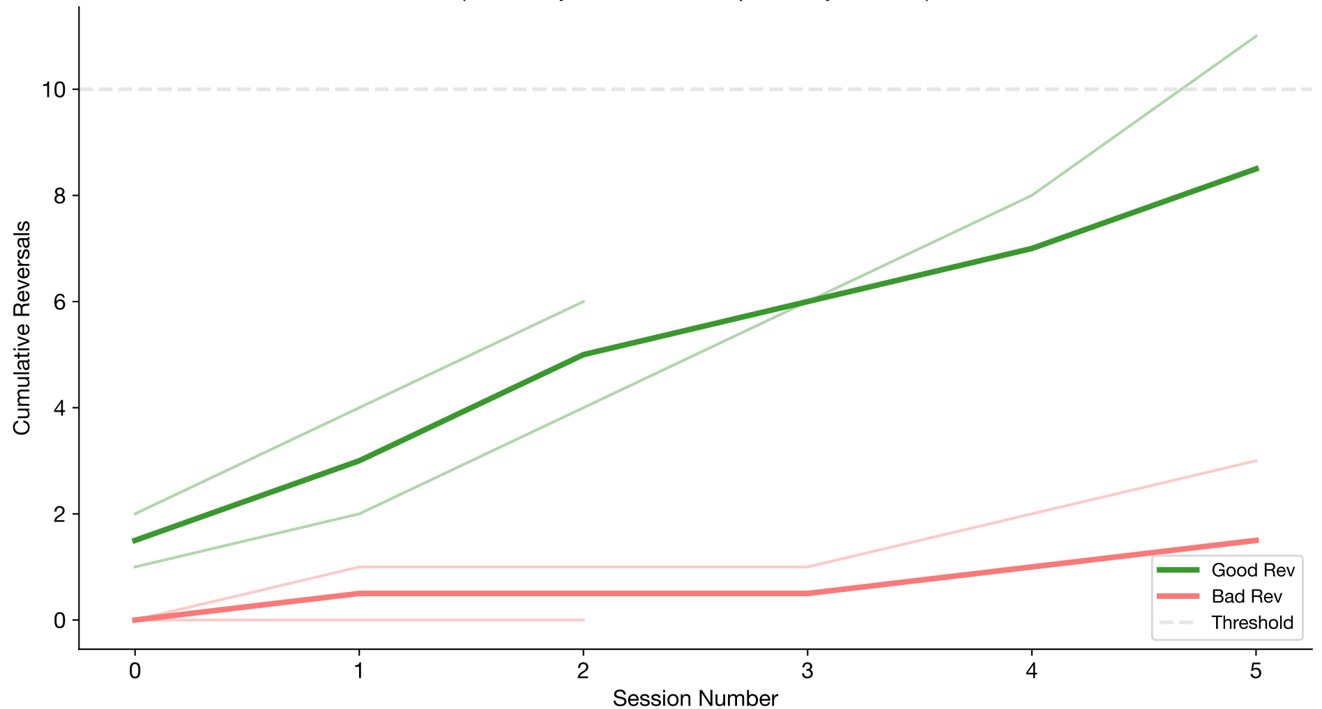
Cumulative Good and Bad Reversals Over Time (n=2 subjects; sessions per subject=3–6)
